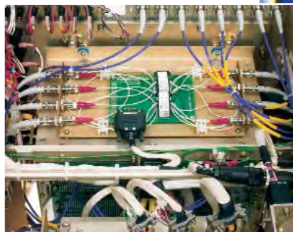
Copper and Fibre Mix
